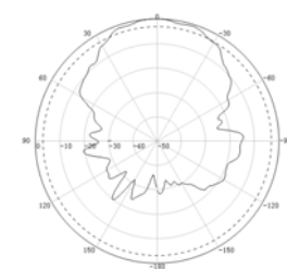
Vertical 3800MHz
