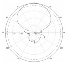
Vertical 960MHz
