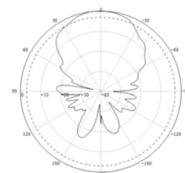
Vertical 1880MHz
