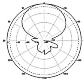
Vertical 960MHz
