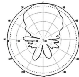
Vertical 1880MHz
