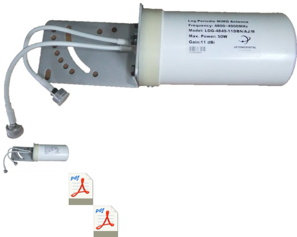
4800-4900MHz Log-Periodic MIMO Antenna(11dbi)
