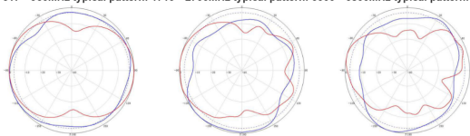
617 ~ 960MHz typical pattern: 1710 ~ 2700MHz typical pattern: 3300 ~ 3800MHz typical pattern:
